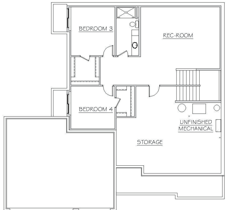
LOWER LEVEL
