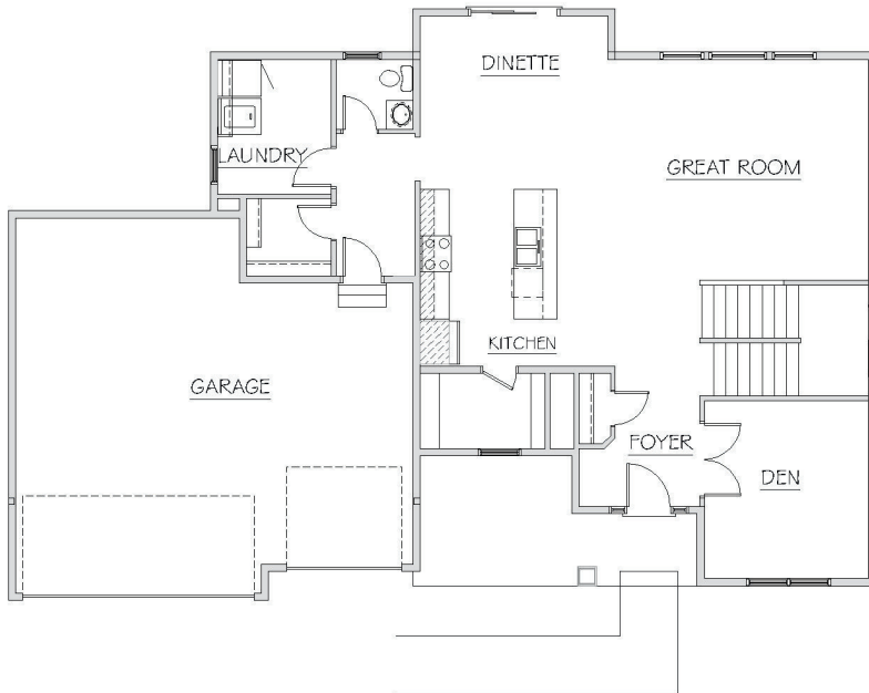
MAIN LEVEL
