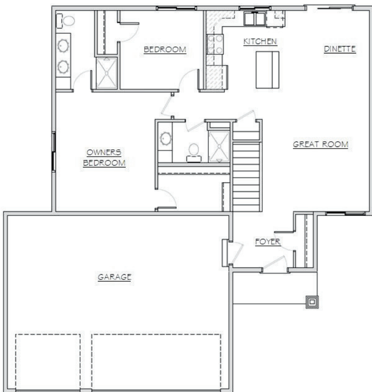
MAIN LEVEL
