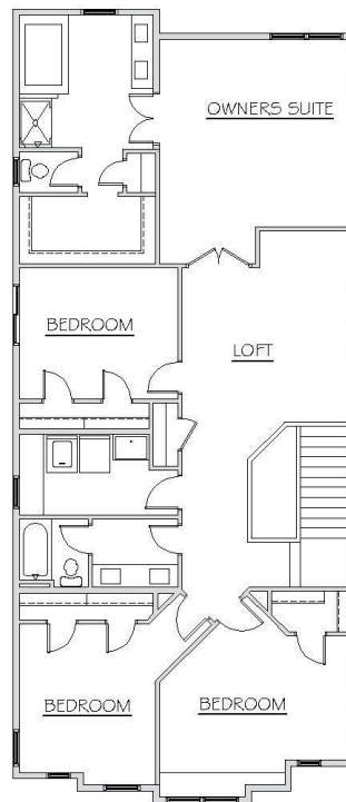
UPPER LEVEL
