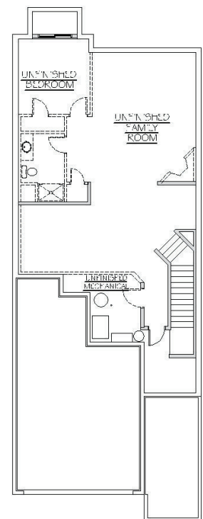
LOWER LEVEL
