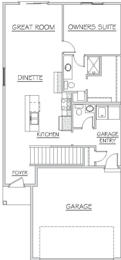
MAIN LEVEL
