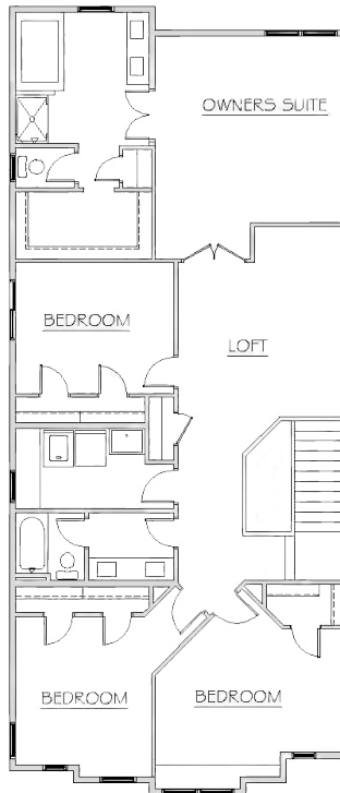
UPPER LEVEL
